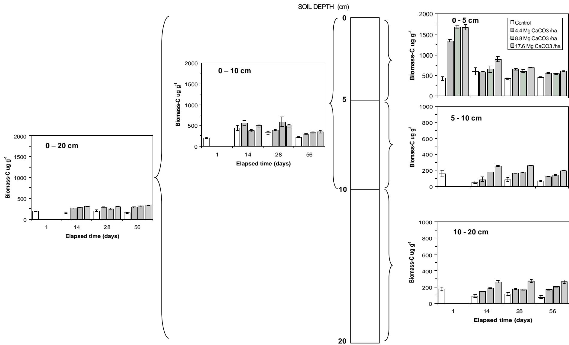
Figure 5: Microbial biomass with different liming rates, incubation times and soil depths estimated by the substrate induced respiration method (SIR) of a 27 year-old No-till system, Palouse, WA (Error bars represent \pm one standard error of the mean, n=4 ).
